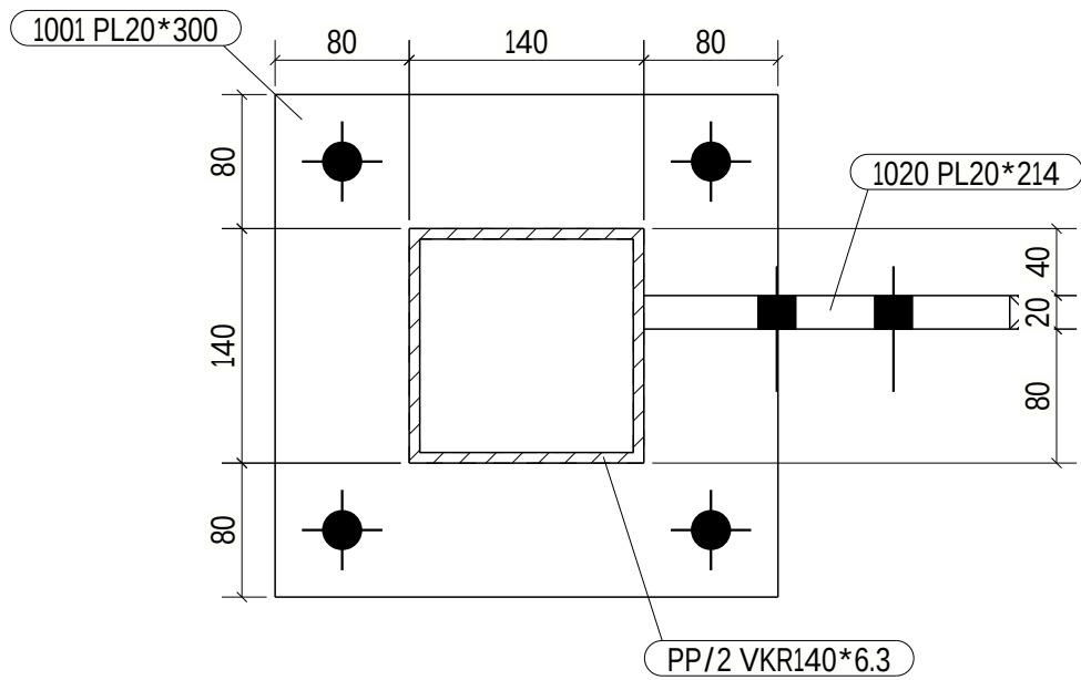
A - A 1:5
